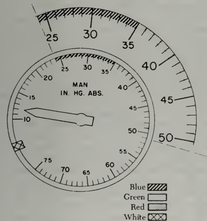
FIGURE 10-25. Manifold pressure gage.
